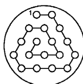
Eighteen (18) Size 22 Contacts
