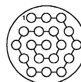
Nineteen (19) Size 20 Contacts
