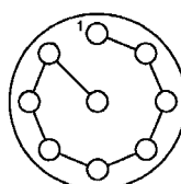
Nine (9) Size 20 Contacts
