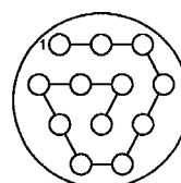
Twelve (12) Size 20 Contacts
