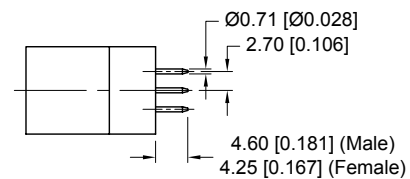
Size 22 contacts
