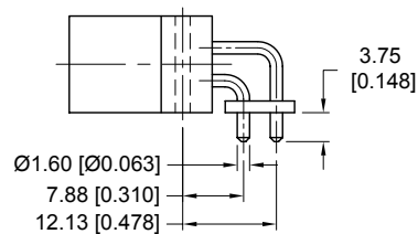
Size 16 contacts
